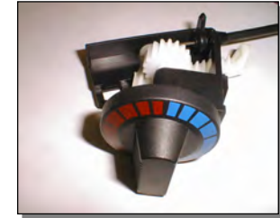
Shown with installed 1.75" dia. temperature knob and snap-in push/pull cable
